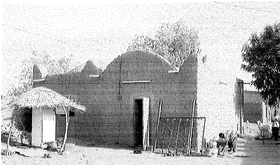
Spontaneous house construction by trained builders in Niger using local available earth bricks.
