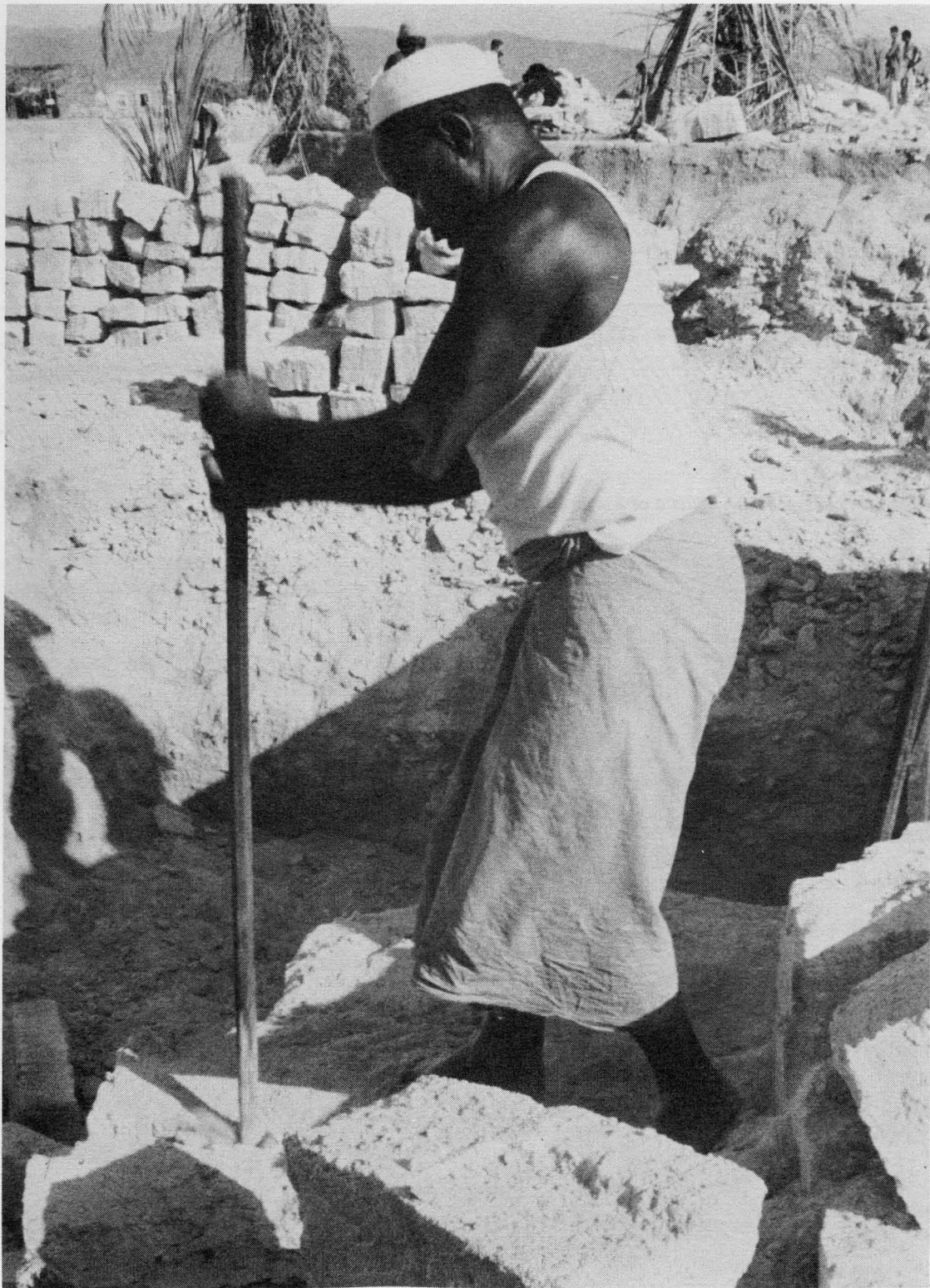
The manual method of quarrying limestone is with pike, hammer and chisel.
