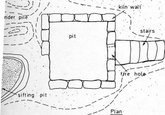
Traditional Nourah-Lime Burning Kiln-Pit in the Salala area.
