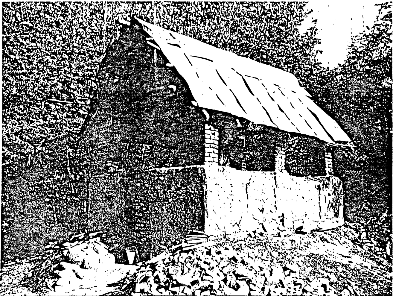
Chubar open top updraught kiln with capacity of 7500 tiles.
