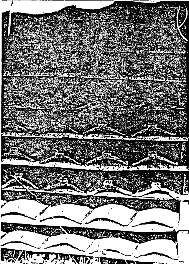
Unfired tiles drying on racks.
