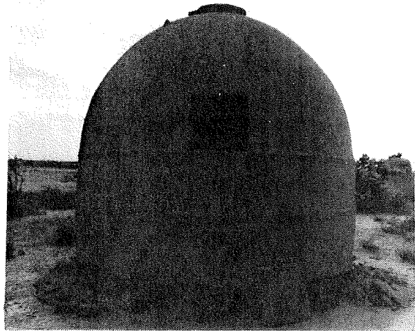
"Coil" construction granary typical of many regions of the Sahel, with thin unstabilized earth walls. Local knowledge of how to ensure that such buildings resist heavy downpours of rain exists...
