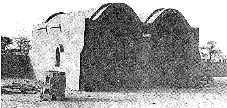
Unstabilized mud brick vaults with an earth render: after 7 years of no maintenance, structurally sound and requiring only re-rendering.
